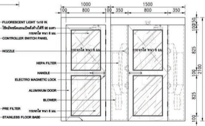
ELEVATION-B SCALE 1:35
