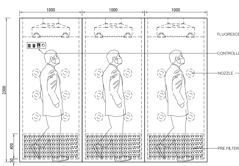
SIDE VIEW SCALE 1:30
