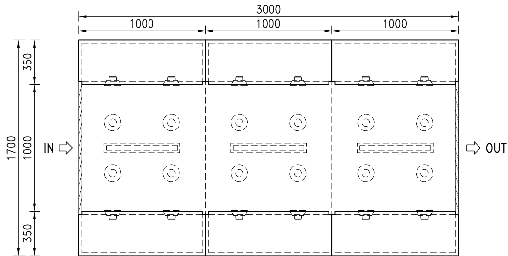
TOP VIEW SCALE 1:30
