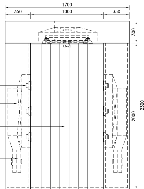
FRONT VIEW SCALE 1:30
